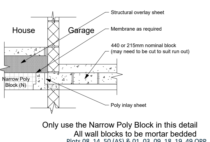
JF155 - Internal Loadbearing Wall (House / Garage)
