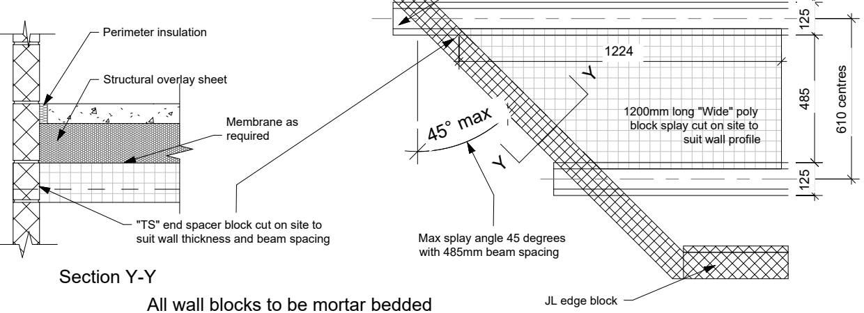
JF128 - Splayed Bearing < 45°, Wide Block
