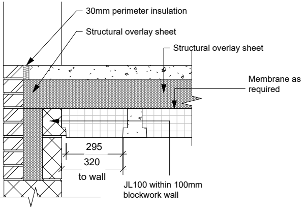
JF157 - Threshold Edge Detail Parallel
