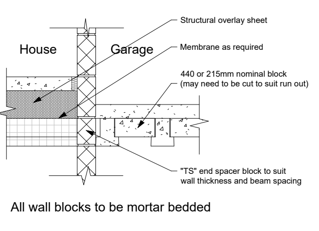
JF154 - Internal Loadbearing Wall (House / Garage)
