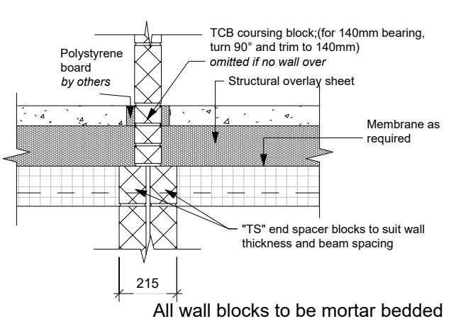
JF126 - End Bearing, min. 215mm Loadbearing Wall
